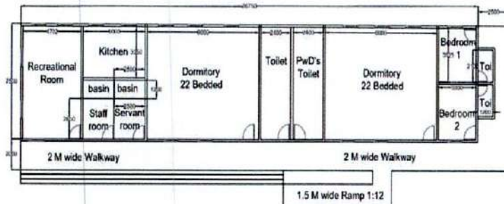
PRIME HUB BLOCK - II (RESIDENTIAL BLOCK) AREA: 372.88 SQM
