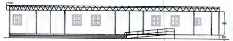
FRONT ELEVATION RESIDENTIAL BLOCK
